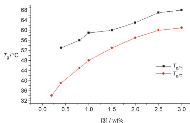
Figure 2. Sol-gel transition temperatures ( T_{g/H} and T_{g/C} ) for gels 3 /DMSO as a function of gelator concentration.
