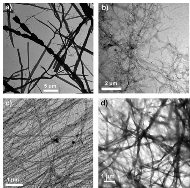
Figure 1. Selected TEM images of gels formed by pincer complex 3 (concentration 1 wt%). a) MeOH; b) DMSO; c) DMF; d) DMA.
