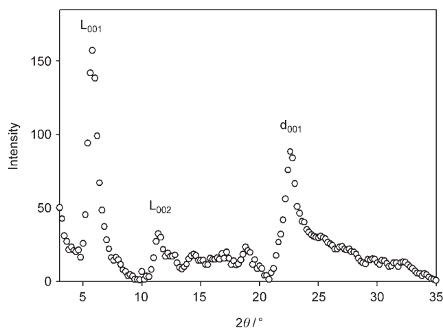
Figure 4. X-ray diffraction pattern of gel 3 /DMSO (3 wt%; after subtraction of the solvent-based background).
