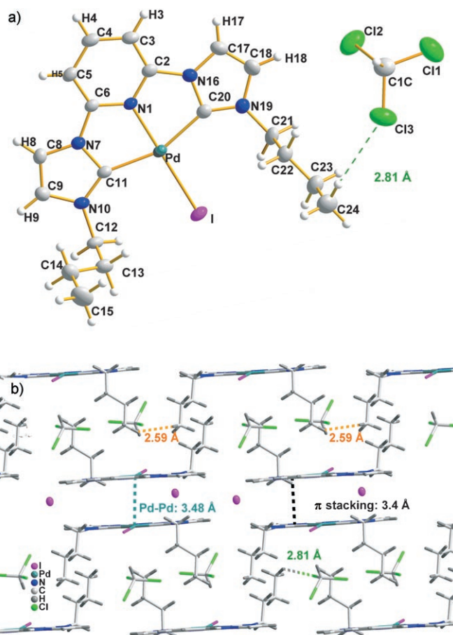
Figure 5. a) Molecular structure of 2b · \text{CHCl}_3 in the crystal. b) View along the a axis showing part of a truncated 2 \times 2 \times 2 array of unit cells.
