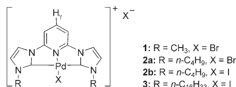
Scheme 1. Palladium CNC pincer bis(carbene) complexes.
