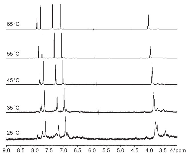
Figure 3. Temperature-dependent ^1\text{H} NMR spectra (aromatic and \text{NCH}_2 alkyl region) of gel 3 /[ \text{D}_6 ]DMSO (1 wt%).
